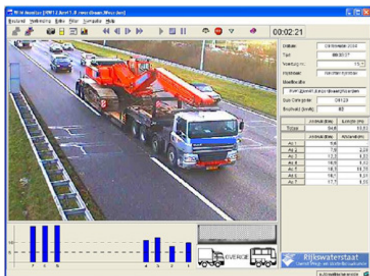
Figure 3.2: Example of data measured by an extended WIM system. Source: RIJKSWATERSTAAT
